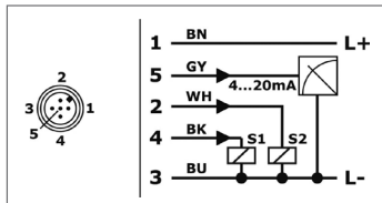
5-wire – output 2x switch PNP / 1x current 4...20mA
