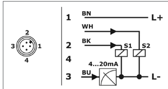
4-wire – output 2x switch PNP
