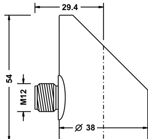
Connection housing
