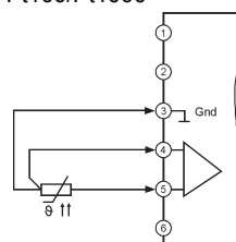
Pt100/Pt1000
